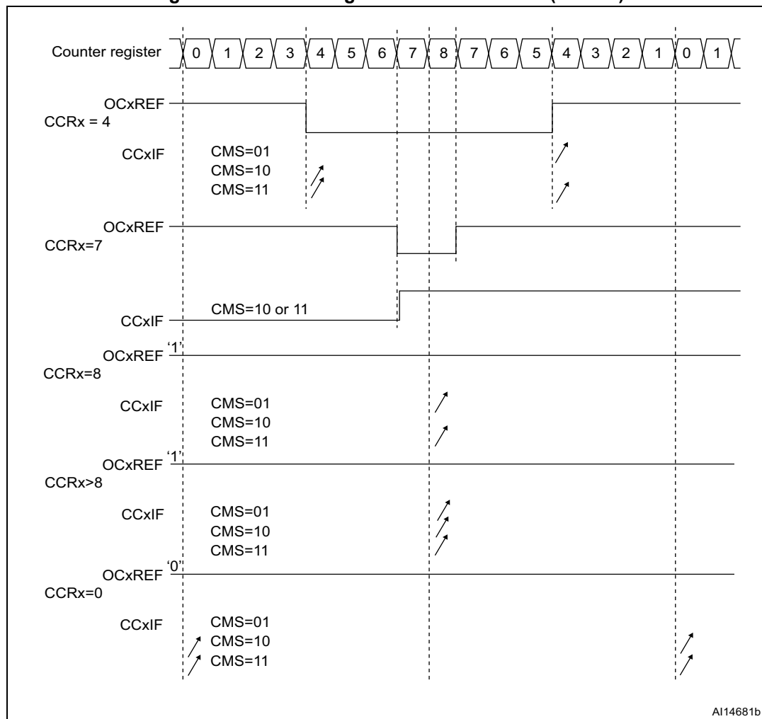
Figure 180. Center-aligned PWM waveforms (ARR=8)
