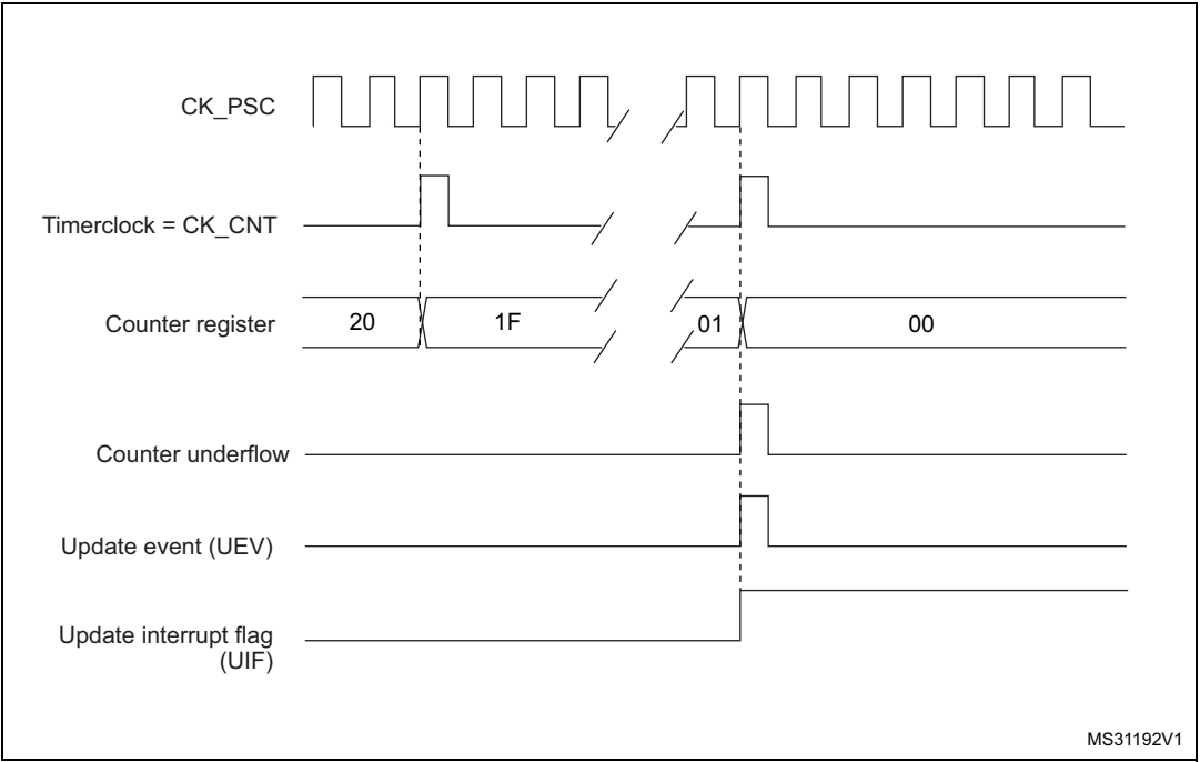
Figure 221. Counter timing diagram, Update event with ARPE=1 (counter underflow)
