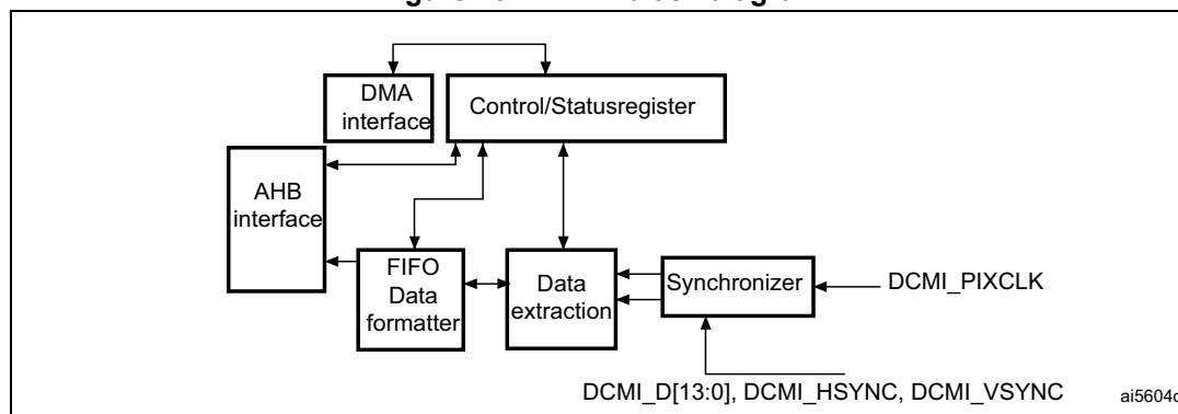
Figure 102. DCMI block diagram
