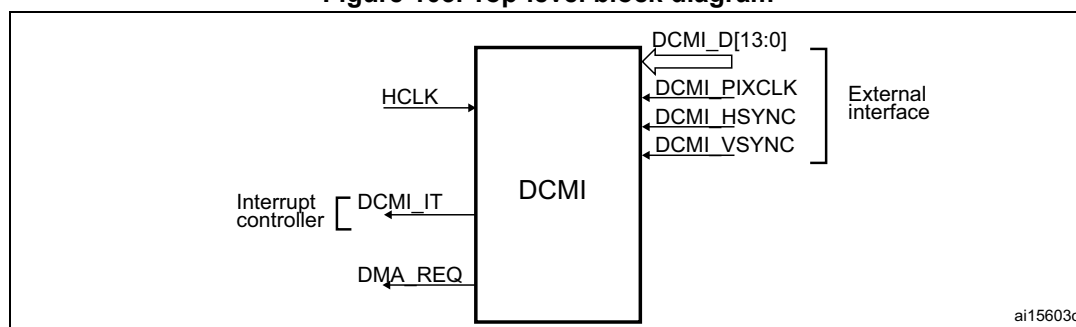
Figure 103. Top-level block diagram
