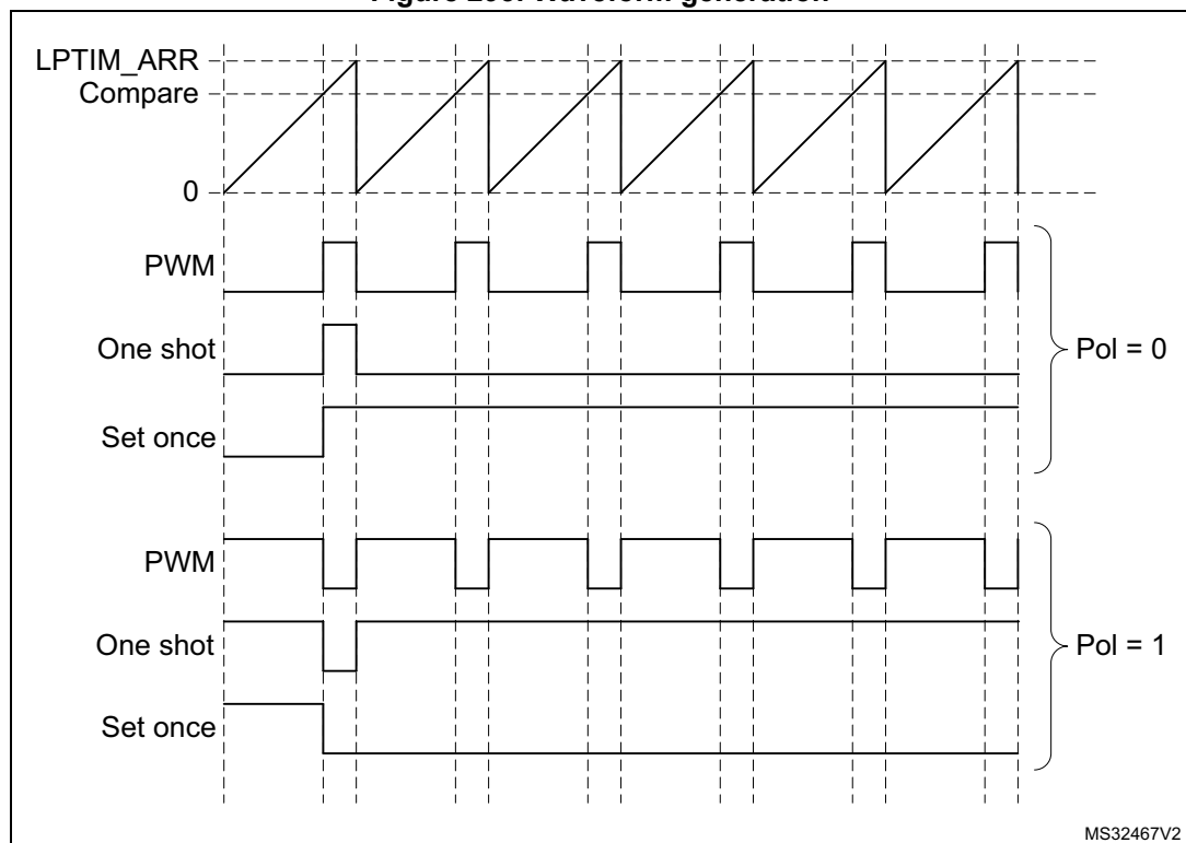
Figure 293. Waveform generation
