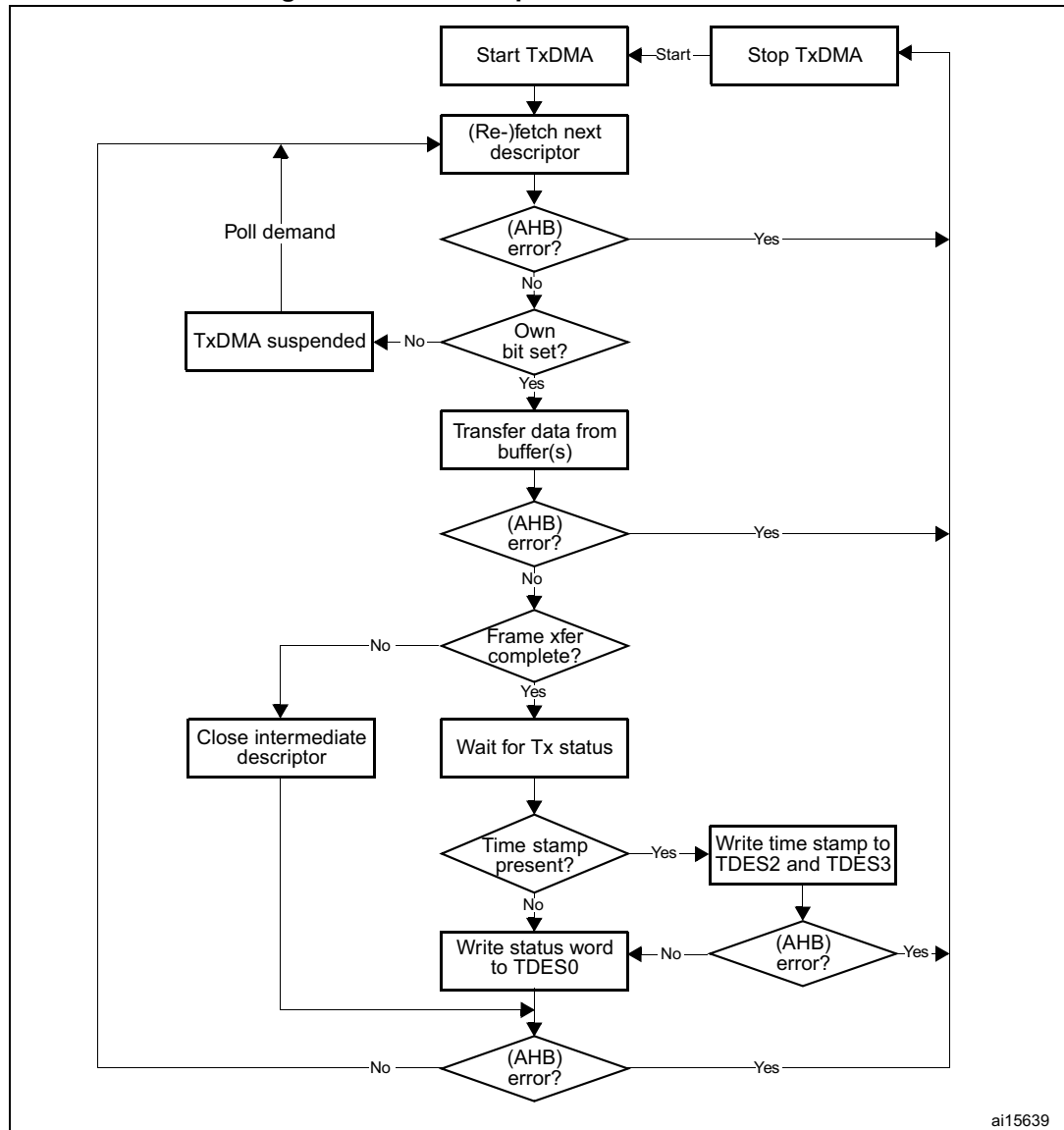
Figure 513. TxDMA operation in default mode
