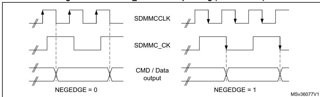
Figure 432. SDMMC_CLK clock dephasing (BYPASS = 0)
