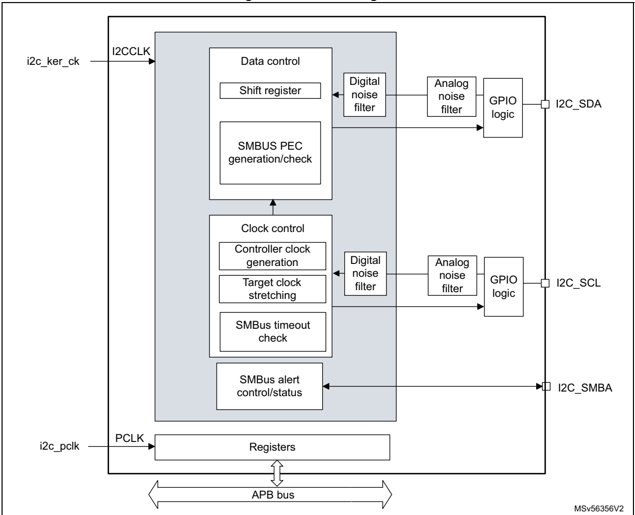
Figure 299. Block diagram
